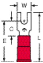
MVU18-4FB/S Stud Size 4 Wire Range 22-18
