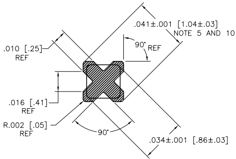
SECTION A-A SCALE 10:1 (FERRULE REMOVED)
