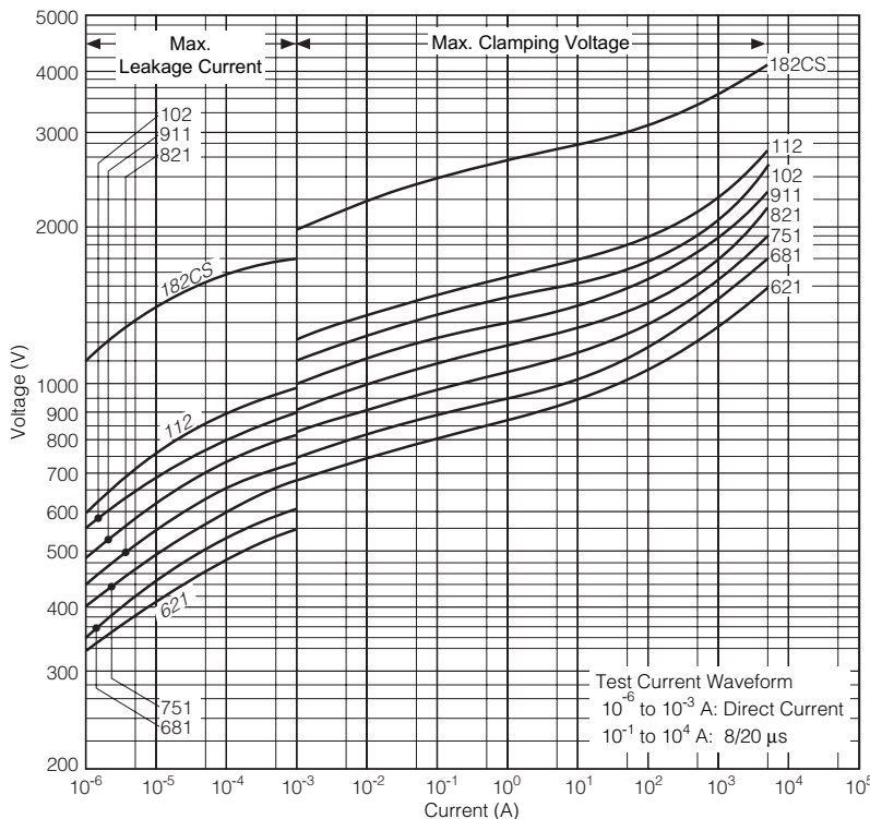
ERZV14D621 to ERZV14D182CS
