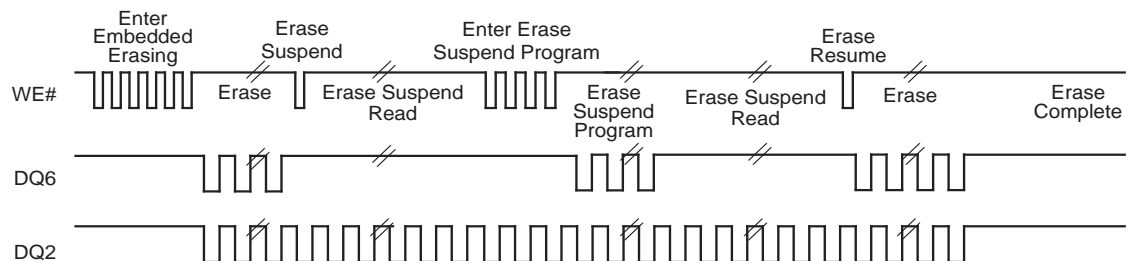
Figure 10.17 DQ2 vs. DQ6 Relationship Diagram
