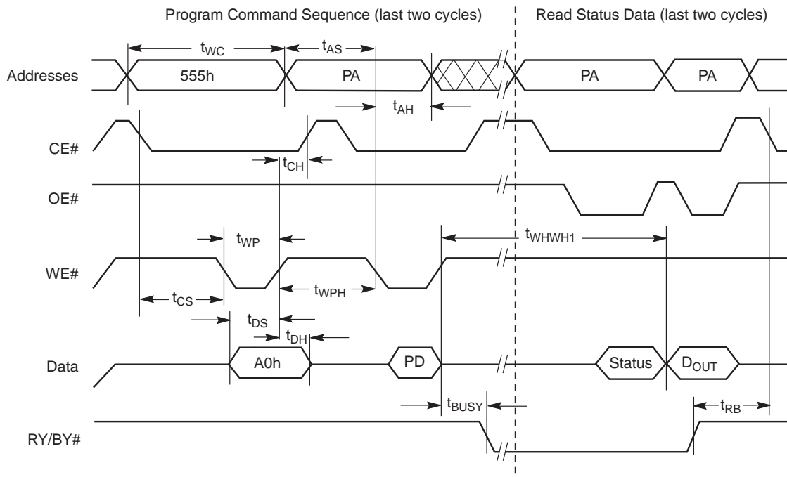
Figure 10.13 Program Operation Timing Diagram
