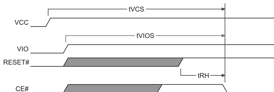
Figure 10.3 Power-Up Diagram
