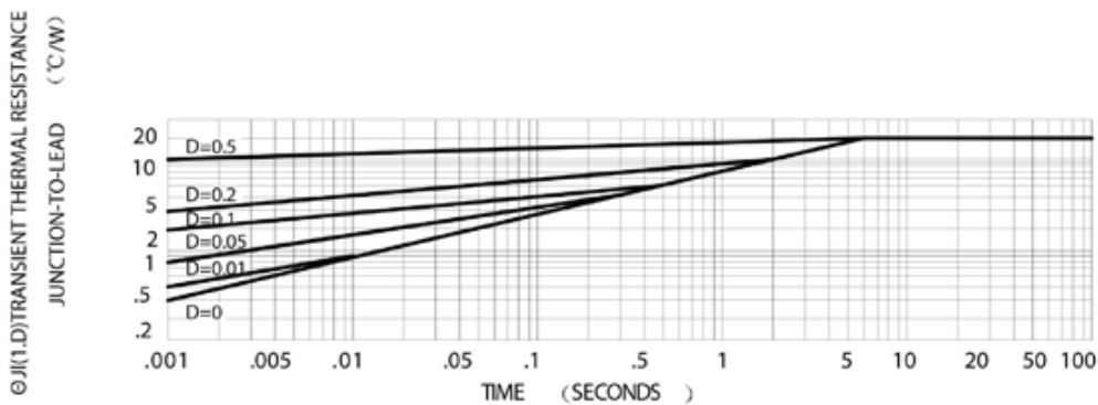
FIG.5 -- TYPICAL THERMAL RESPONSE
