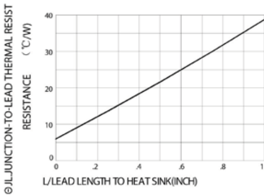
FIG.5 -- TYPICAL THERMAL RESPONSE
