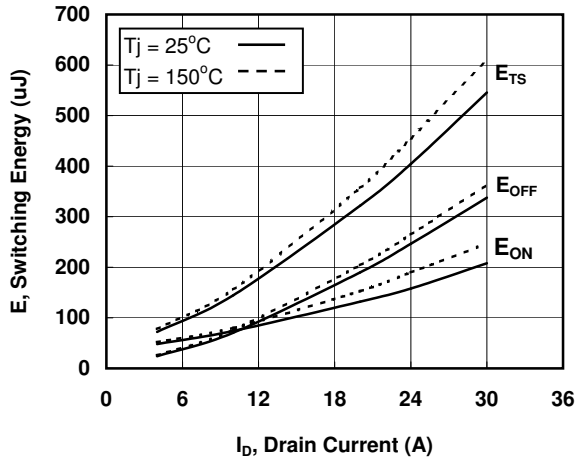
Figure 13. Switching Energy Losses
