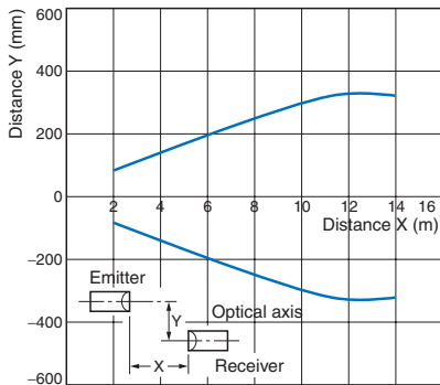
Parallel Operating Range (Typical) Through-beam E3JM-10□4(T)
