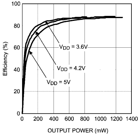
EFFICIENCY vs OUTPUT POWER R_L = 8\Omega , f = 1\text{kHz} , Loudspeaker Mode 2
