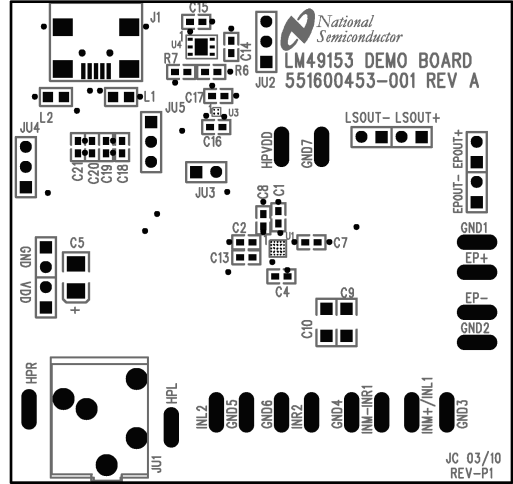
Top Silkscreen
