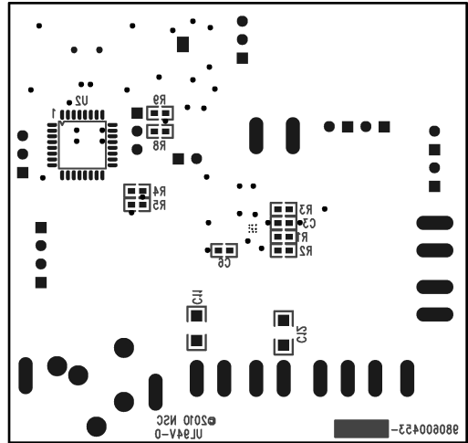
Bottom Silkscreen
