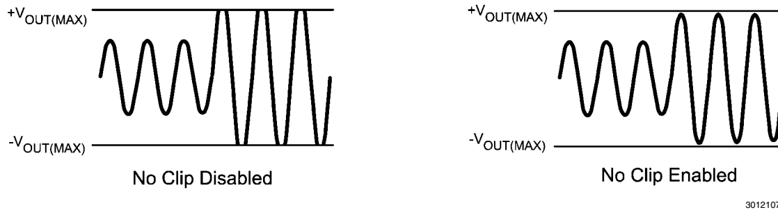
FIGURE 5. No Clip Function
