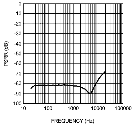
PSRR vs FREQUENCY V_{DD} = 3.6V , HPV_{DD} = 1.8V , HPV_{DD-RIPPLE} = 200mV_{P-P} R_L = 32\Omega , Mono Input, HP Mode
