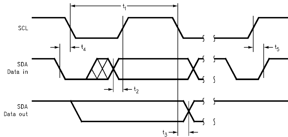
FIGURE 2. I 2 C Timing Diagram
