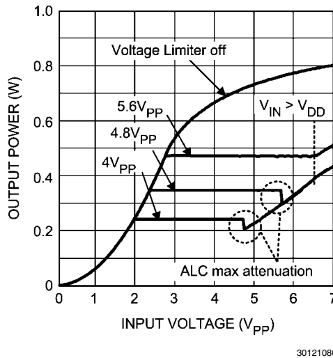
FIGURE 7. Voltage Limiter Function
