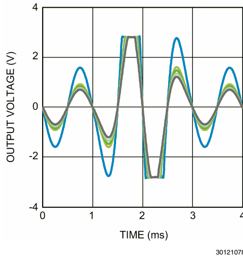
FIGURE 6. Clip Control Levels
