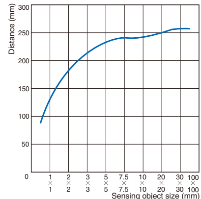
Sensing Object Size vs. Sensing Distance
