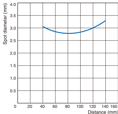
Spot Diameter vs. Sensing Distance
