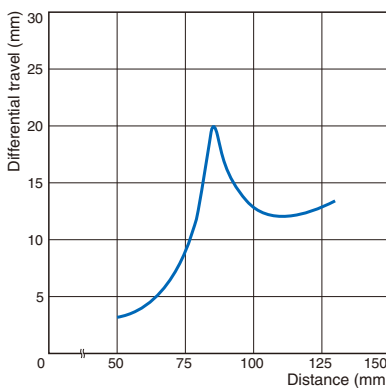
Differential Travel vs. Sensing Distance
