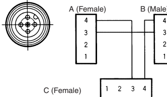
Internal Connections
