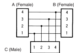
Internal Connections
