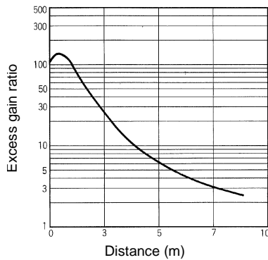
Excess Gain vs. Set Distance (Typical) E3S-ATj 1
