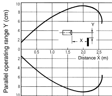
Reflector Parallel Movement (Typical) E3S-ARj 1
