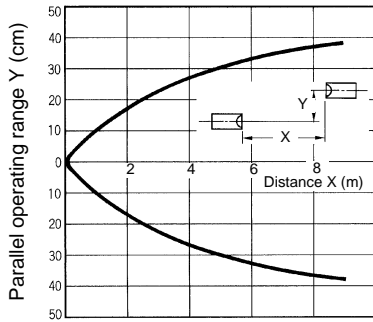
Parallel Operating Range (Typical) E3S-ATj 1
