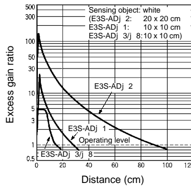
E3S-ADj 1, -ADj 2, -ADj 3, -ADj 8 (Detection of White Paper) E3S-ADj 1, -ADj 2, -ADj 3, -ADj 8 (Detection of Black Paper)
