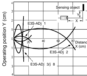
Operating Range (Typical) E3S-ADj (Left and Right)
