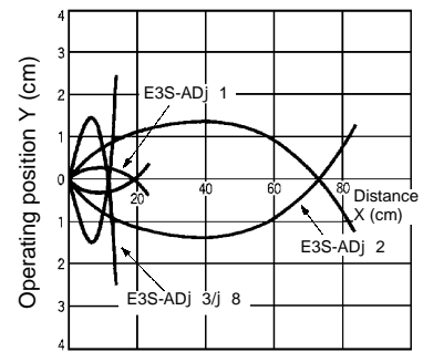
E3S-ADj (Up and Down)
