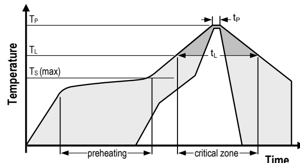
Figure 9 Soldering profile according to JEDEC standard. T_P <= 260^\circ\text{C} and t_P < 30\text{sec} for Pb-free assembly. T_L < 220^\circ\text{C} and t_L < 150\text{sec} . Ramp-up/down speeds shall be < 5^\circ\text{C}/\text{sec} .
