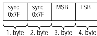
Figure 8: Byte sequence of one value
