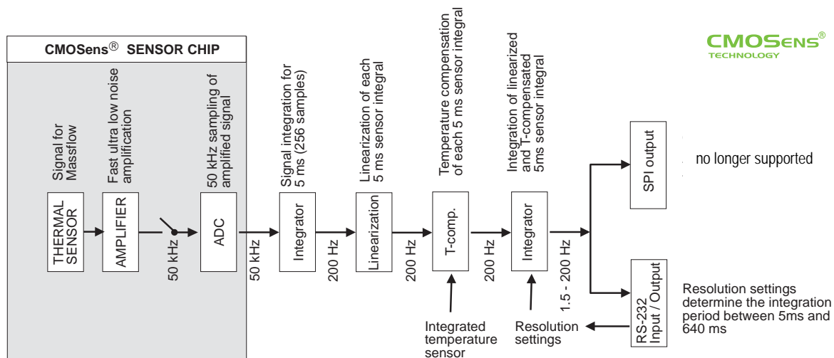
Figure 1: Block Diagram ASF1430 Mass Flow Sensor.
