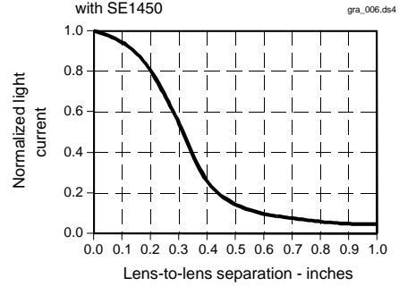
Fig. 6 Coupling Characteristics with SE1450
