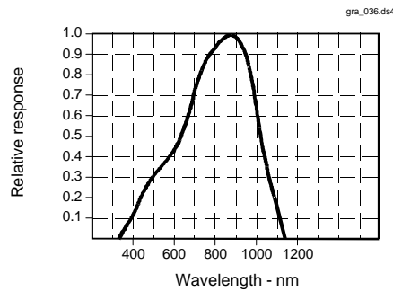
Fig. 3 Spectral Responsivity
