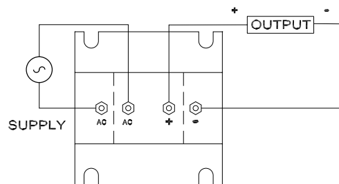
CR4340 100 - 600 Aac
