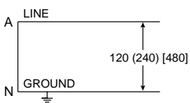
120 V, 2 W (240 V, 2 W) [480 V, 2 W] TWO-WIRE
