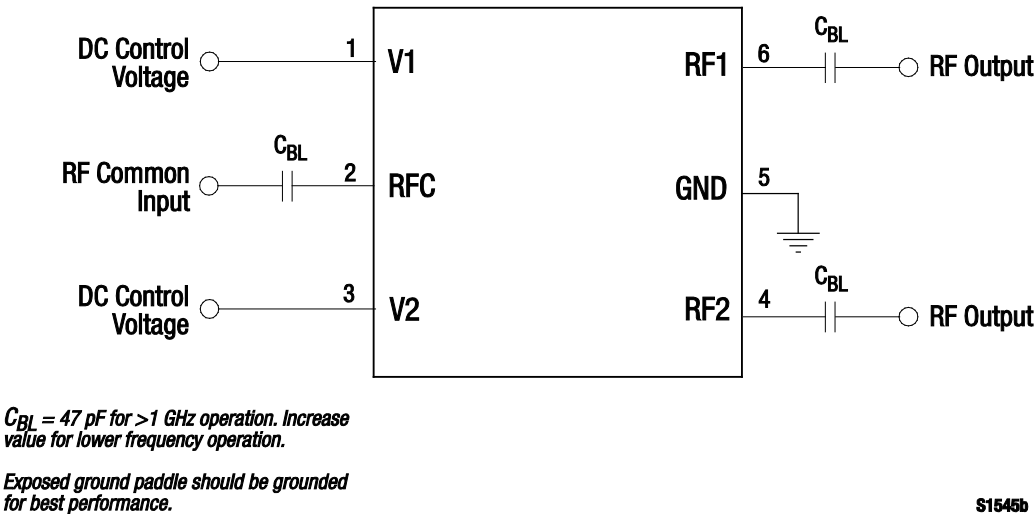
Figure 7. SKY13370-374LF Evaluation Board Schematic
