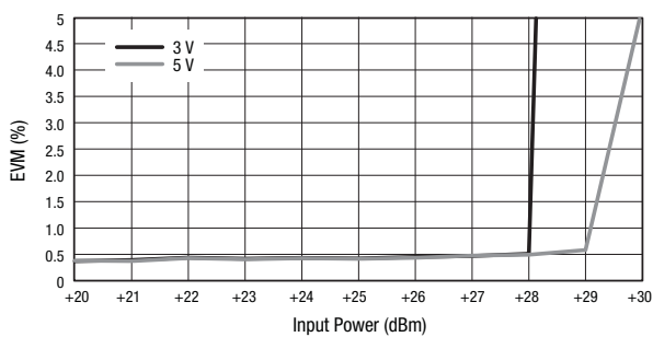
Figure 7. EVM vs Input Power (WiMAX 802.16 64QAM OFDMA, f = 3.8\text{ GHz} )
