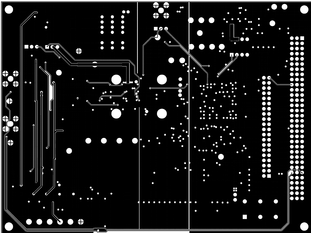
Figure 8. Shield Layer
