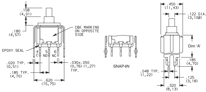
8221SD3_GE DPDT
