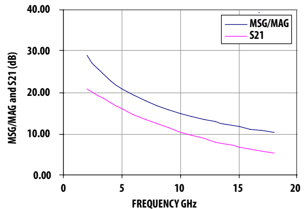
Figure 13. MSG/MAG and S21 vs. Frequency at 1.5V 20 mA
