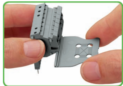
Snapping on a strain relief plate
