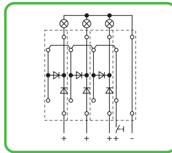
Lamp test circuit
