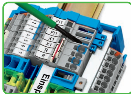
Operation of the slide link using a simple screwdriver
