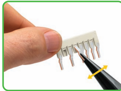
Staggered jumper with 7 contacts Breaking off contact lugs
