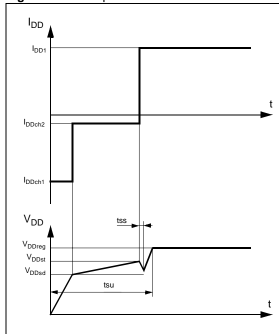
Figure 17: Startup Waveforms
