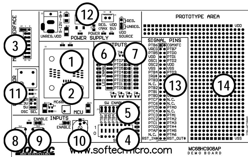
The IDB-HC08AP Demo Board
