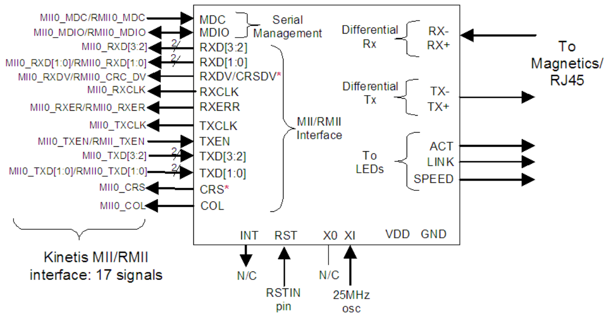
Figure 12-3. MII connection
