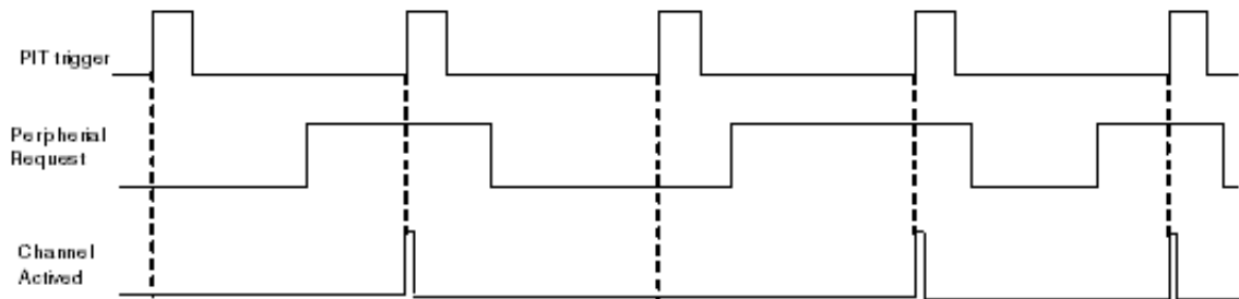
Figure 7-4. PIT gated transfer activation
