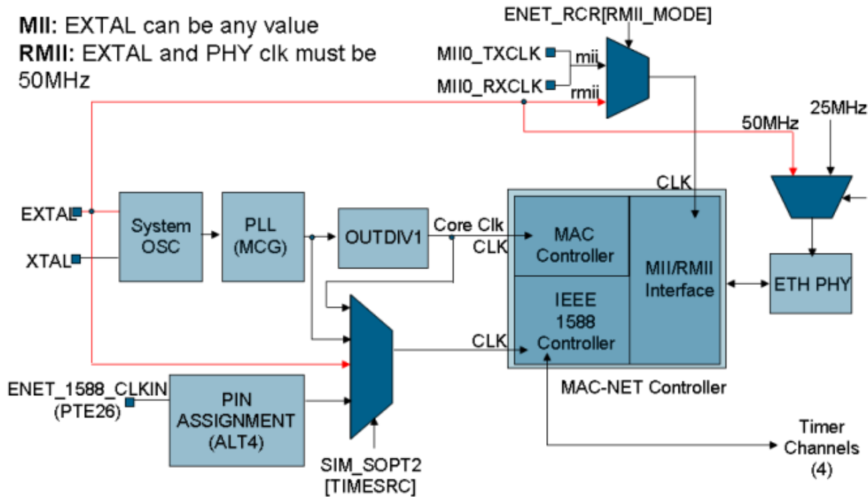
Figure 12-2. MAC-NET interfaces
