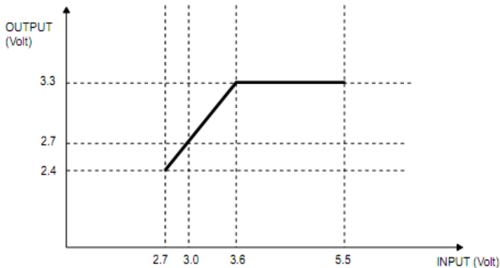
Figure 14-4. Regulator output
