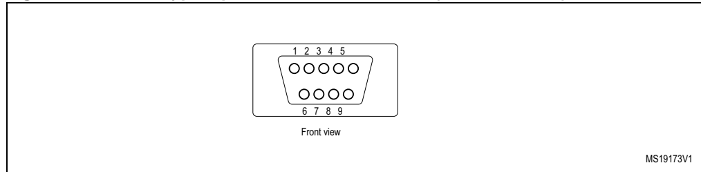
Figure 10. CAN D-type 9-pin male connector CN10 (CAN1 or CAN2)
