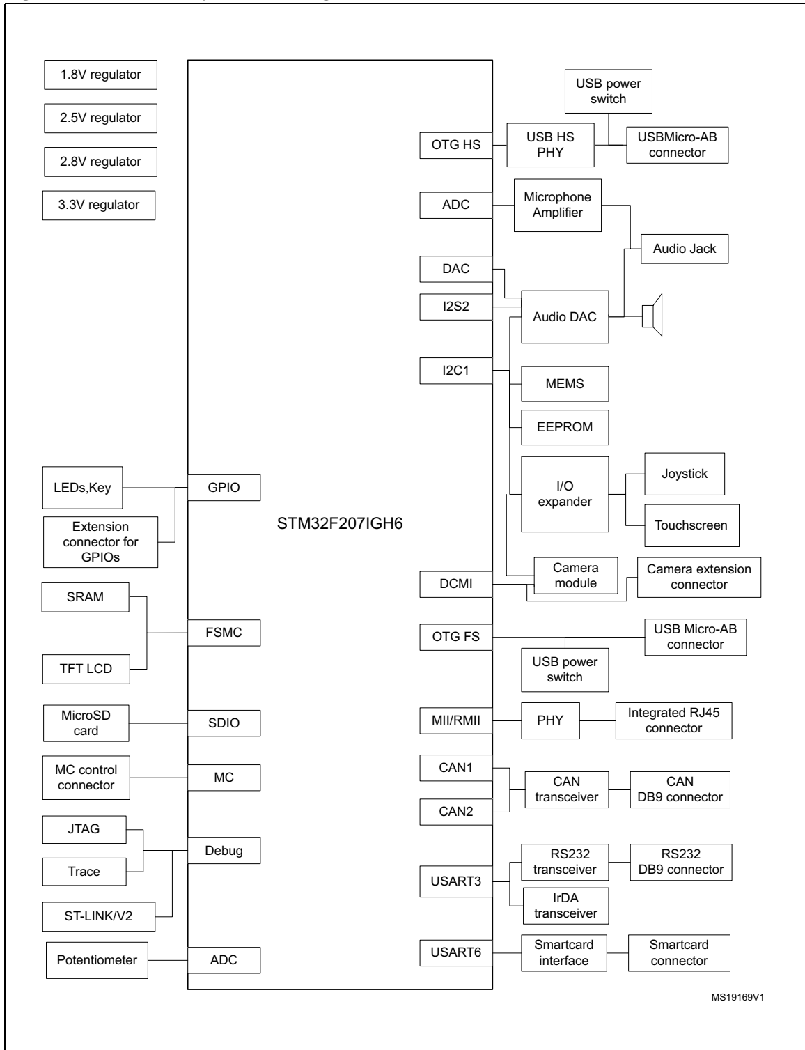
Figure 2. Hardware layout and configuration
