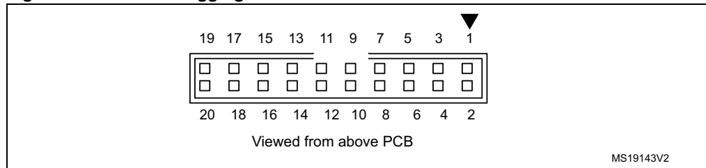
Figure 11. Trace debugging connector CN13
