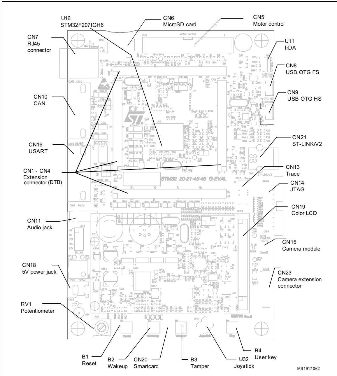
Figure 3. STM3220G-EVAL evaluation board layout
