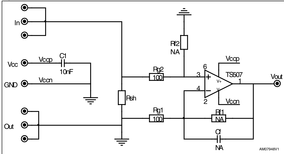
Figure 1. Internal schematic
