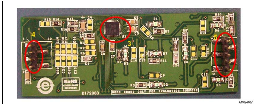
Figure 5. STEVAL-CBP007V1 rear view
