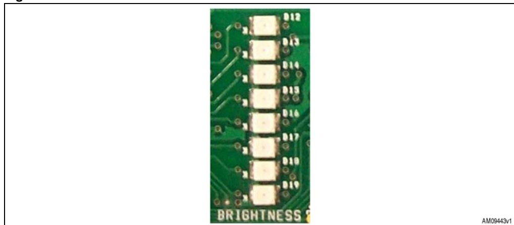
Figure 9. Discrete LEDs
