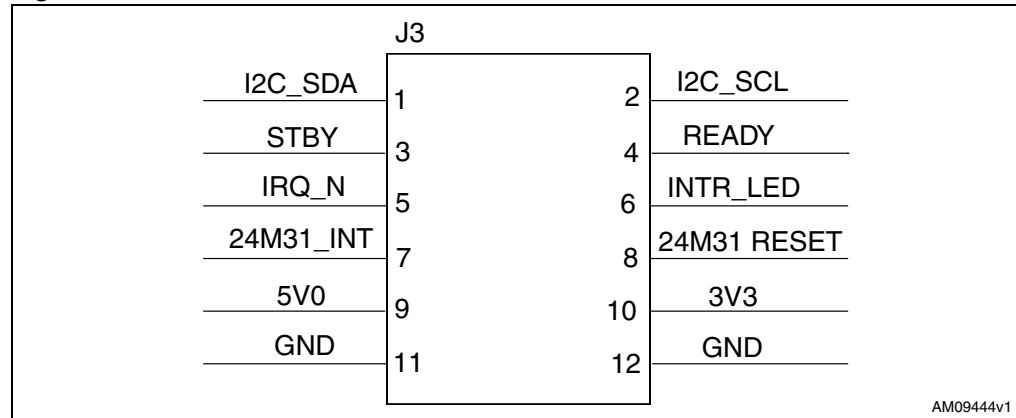
Figure 10. External interface connector
