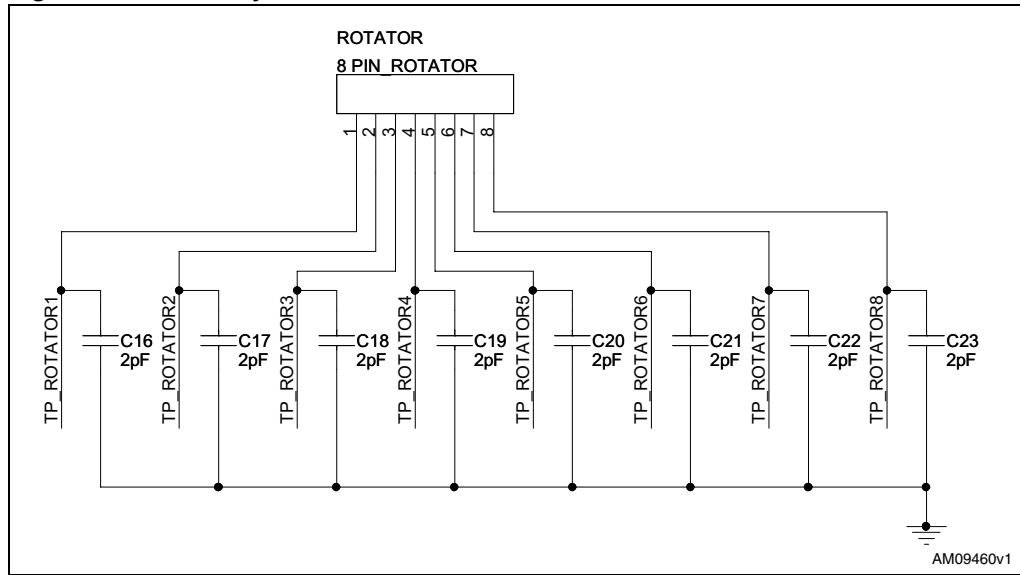
Figure 26. Touchkeys for rotator
