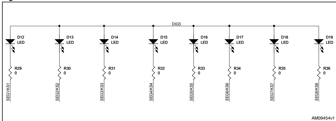
Figure 20. Discrete LED
