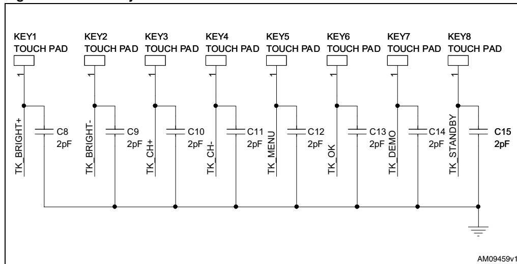
Figure 25. Touchkeys
