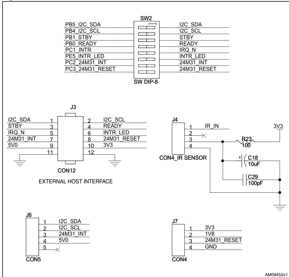
Figure 18. Connectors
