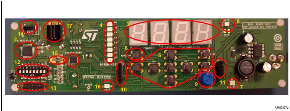
Figure 3. STEVAL-ILL029V2 demonstration board rear view
