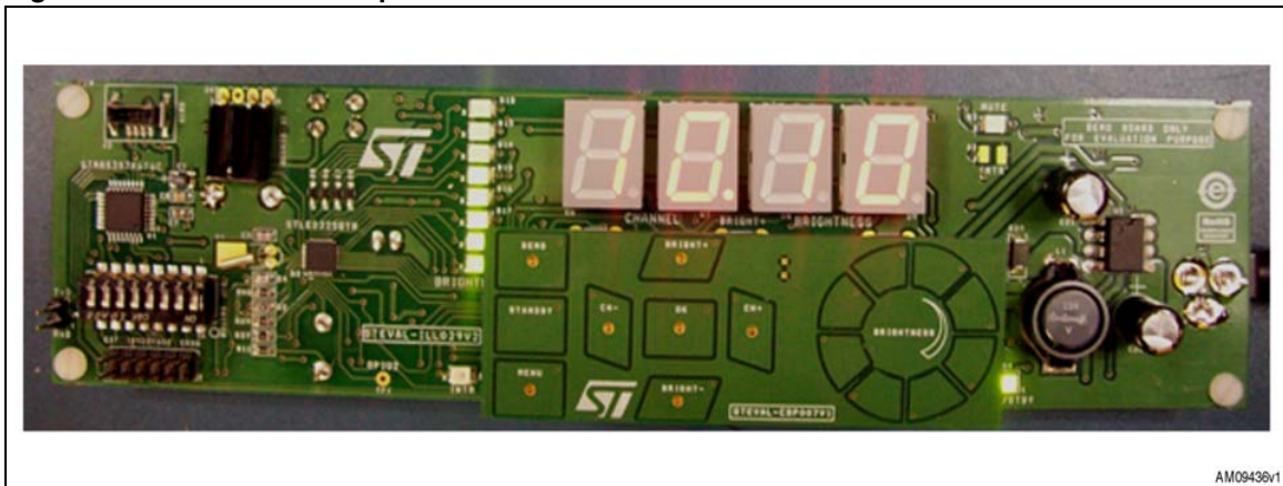
Figure 1. STLED325 front panel demo with STMPE24M31 touch interface
