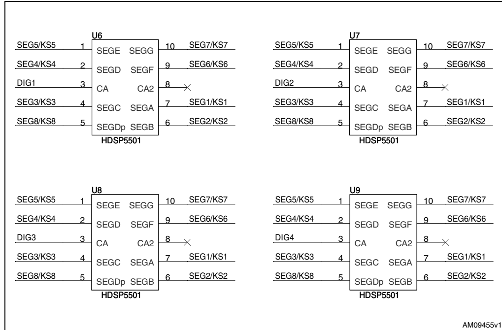
Figure 21. Seven segment LED
