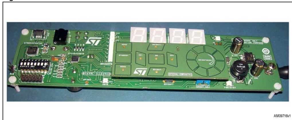
Figure 6. STLED325 board with STEVAL-CBP007V1
