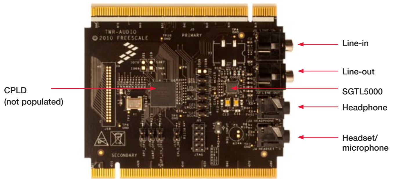
Figure 1: Front Side of TWR-AUDIO-SGTL Module.
