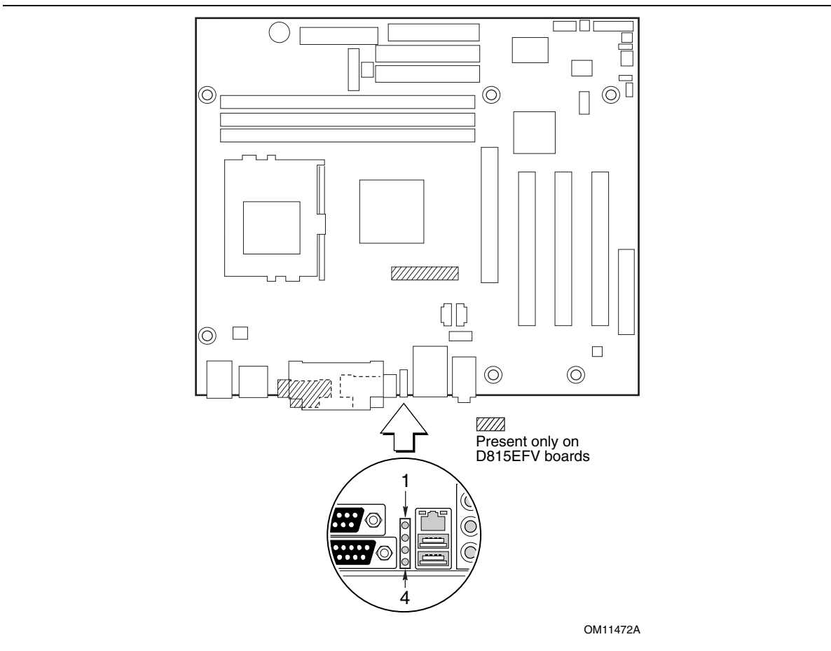
Figure 26. Diagnostic LEDs
