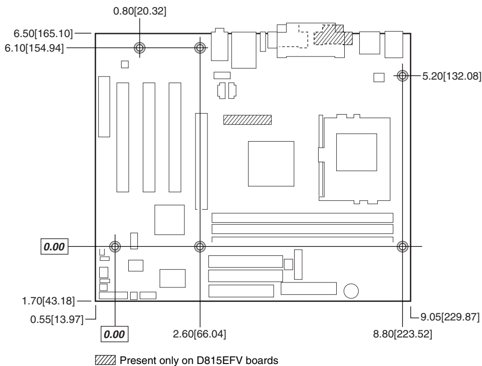
Figure 18. Board Dimensions
