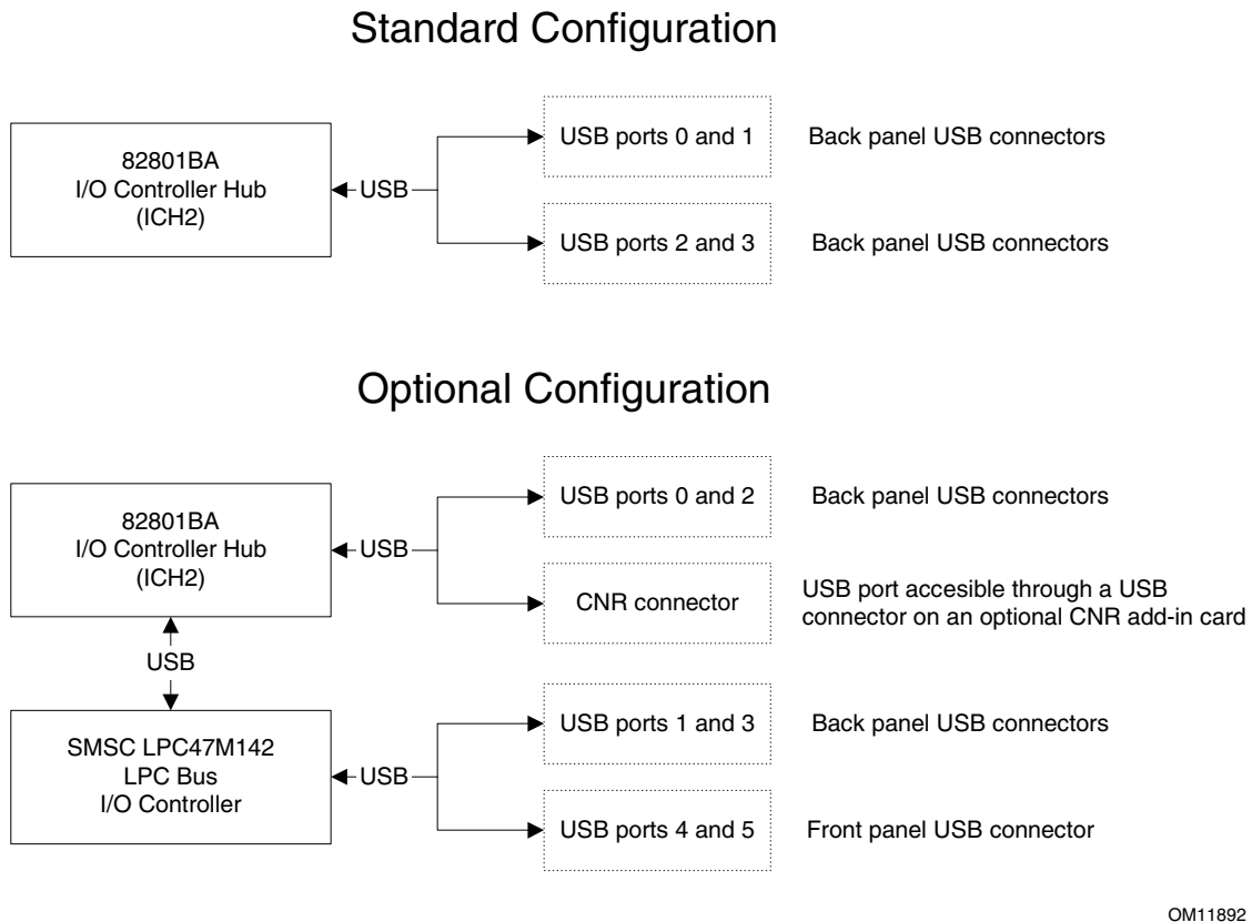
Figure 8. USB Port Configurations
