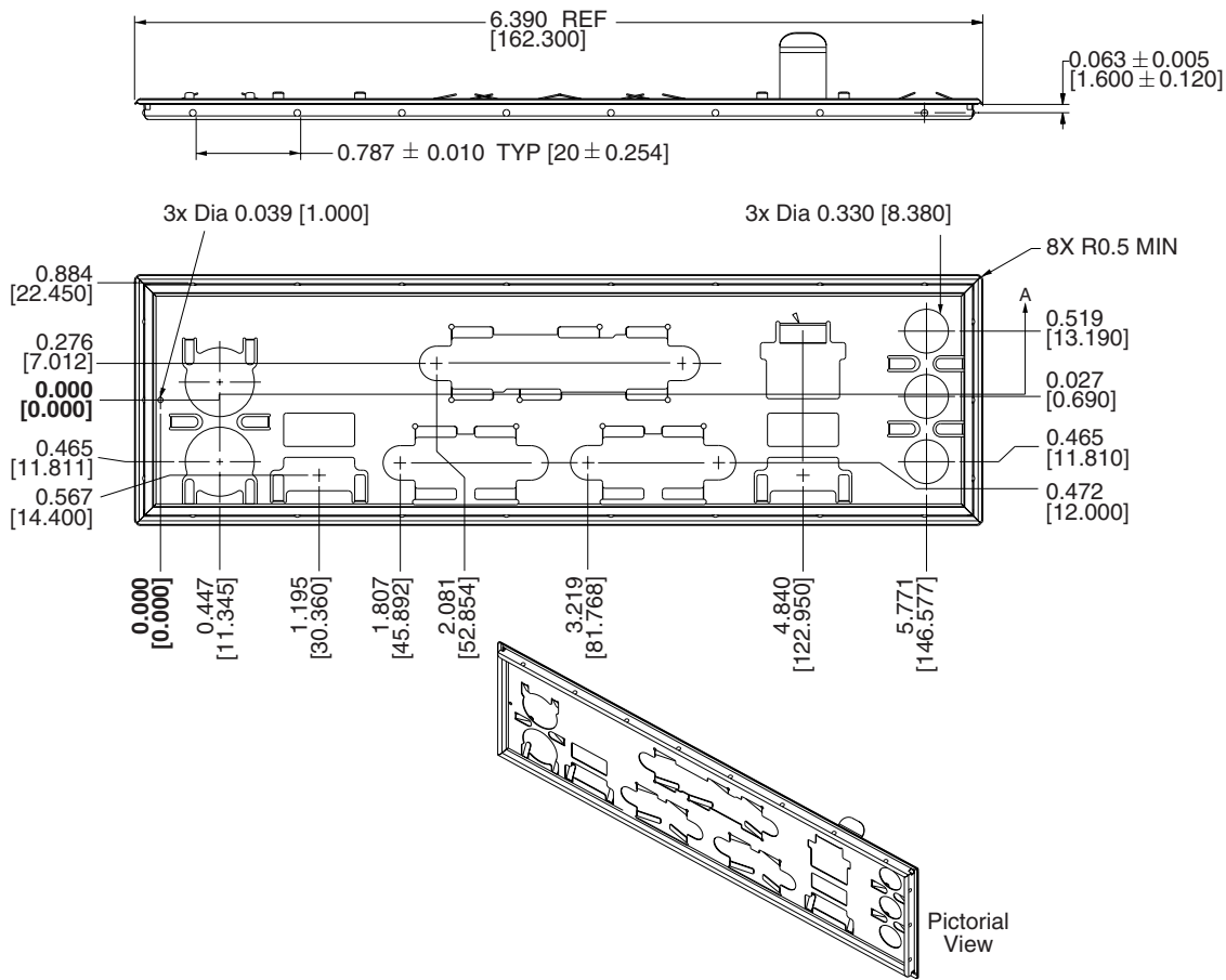
Figure 22. I/O Shield Dimensions (for D815EFV Boards with Onboard LAN Subsystem)
