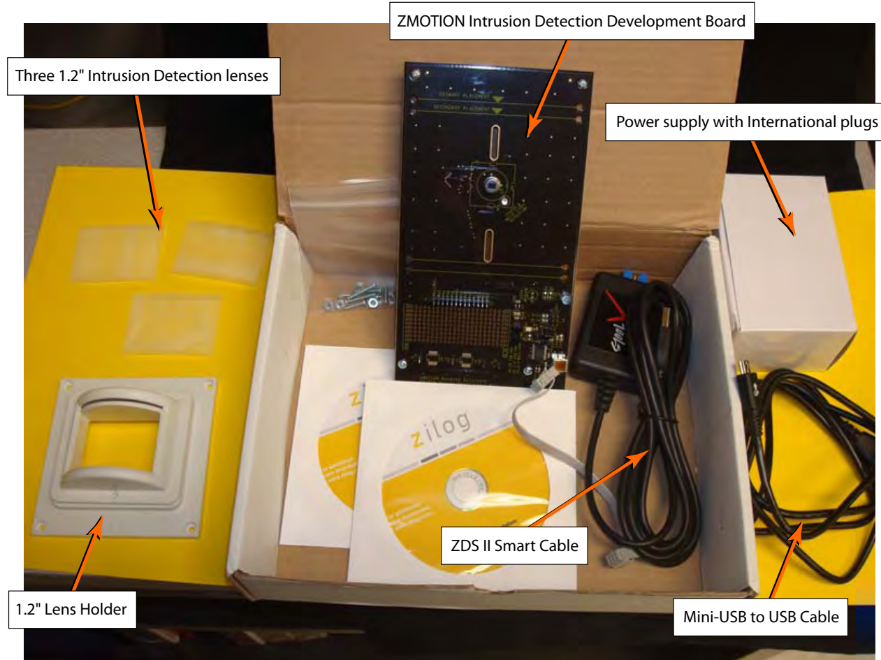
Figure 1. ZMOTION Intrusion Detection Development Kit Components
