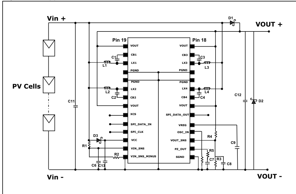
Figure 1. Application circuit
