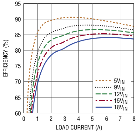
Figure 2. Measured Efficiency on Channel 1 ( V_{OUT1} = 1.5V , f_{SW} = 400kHz , Channel 2 Disabled)
