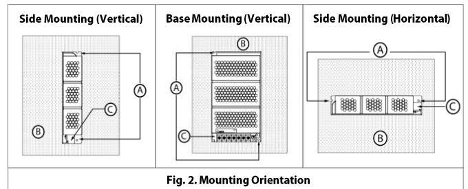
Fig. 2. Mounting Orientation
