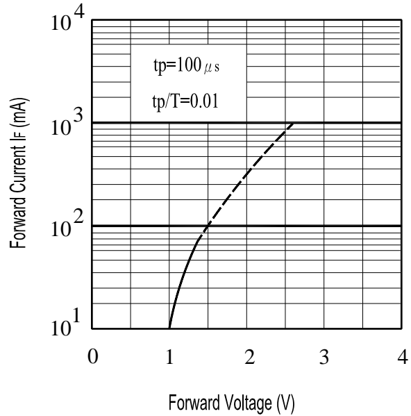
Fig.4 Forward Current
