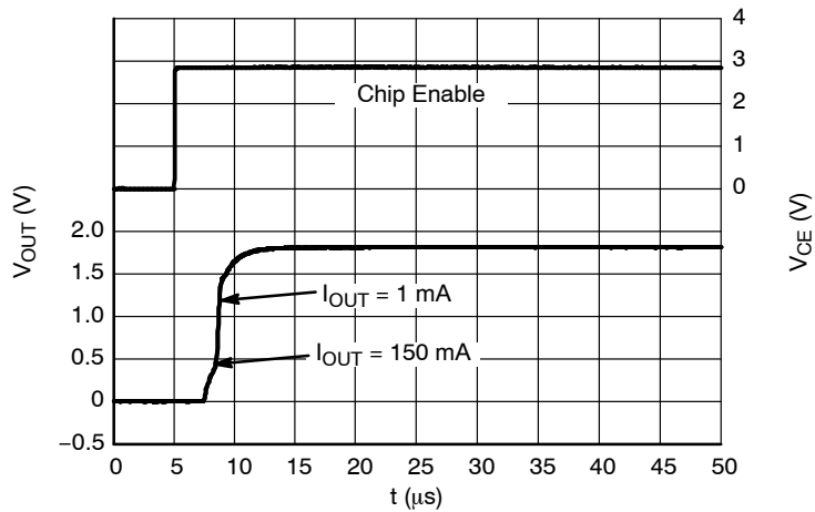
Figure 48. Start-up, 1.8 V Version, V_{IN} = 2.8 V
