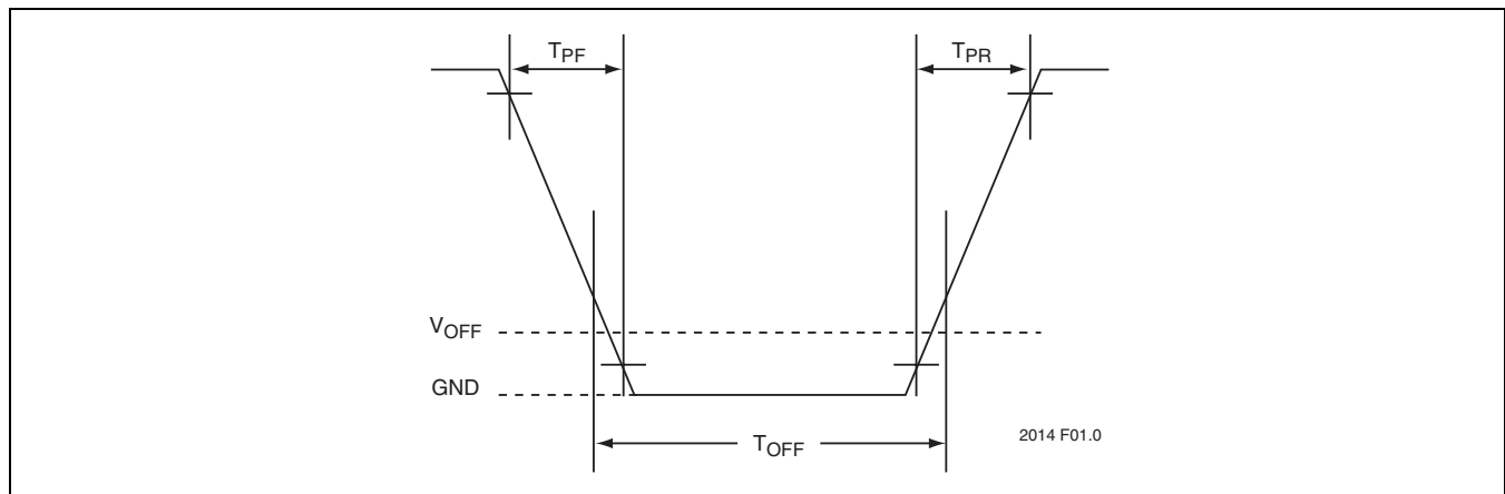
FIGURE 1: RECOMMENDED POWER-UP/DOWN WAVEFORM
