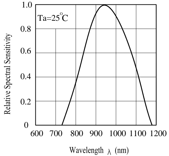
Fig.2 Spectral Sensitivity
