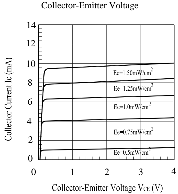
Fig.6 Collector Current vs.
