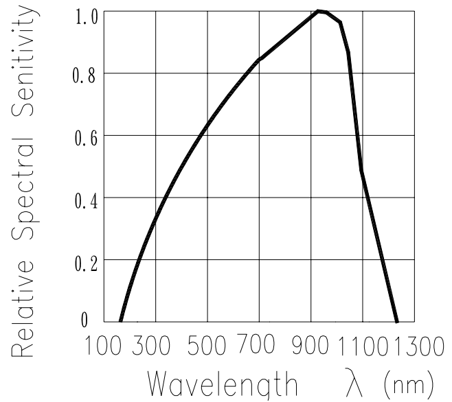
Fig.2 Spectral Sensitivity Ta=25°C
