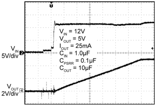
Time (100μs/div)
