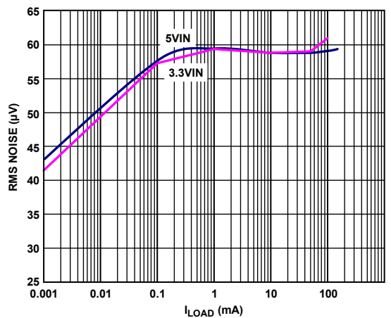
Figure 38. LDO Output Noise vs. Load Current, Across Input Voltage, V_{OUT3} = 3.0\text{ V}
