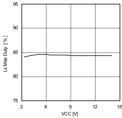
Fig.16. Lx Max duty power supply property
