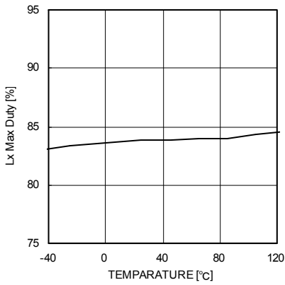
Fig.15. Lx Max duty temperature property
