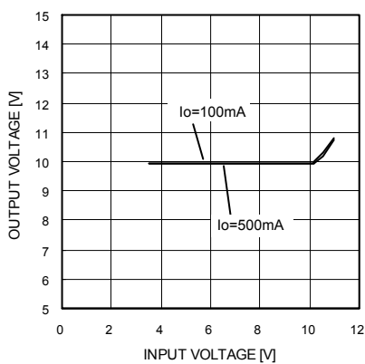
Fig.23 Line regulation
