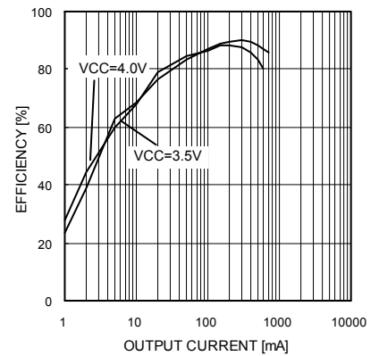
Fig.22 Power conversion efficiency 3
