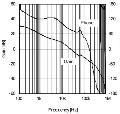
Fig.26 Frequency response property 1 (VCC = 3.0 V, Io = 200 mA)
