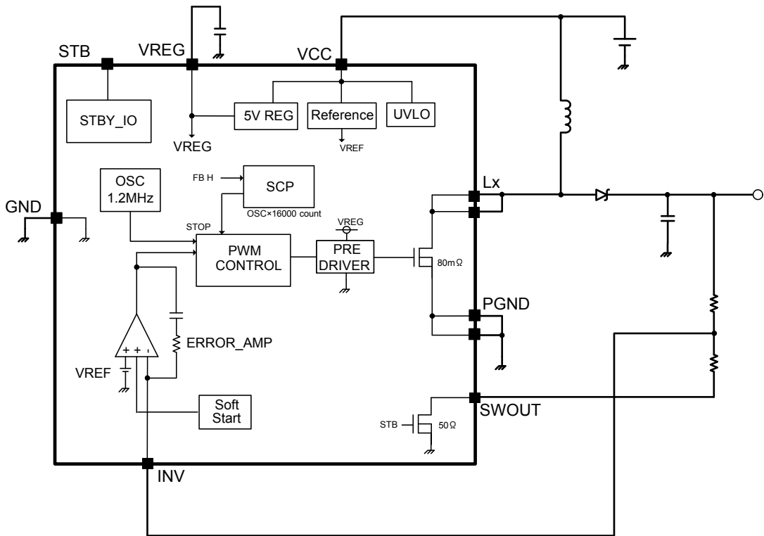
Fig.2 Block diagram
