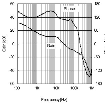
Fig.27 Frequency response property 2 (VCC = 6.0 V, Io = 200 mA)
