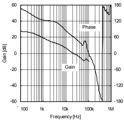
Fig.29 Frequency response property 4 (VCC = 3.0 V, Io = 500 mA)
