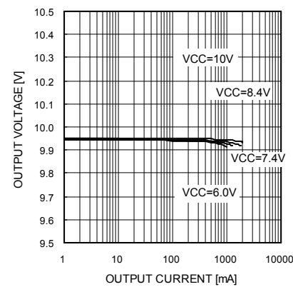
Fig.24 Load regulation 1
