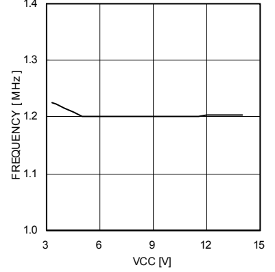
Fig.8. fosc voltage property
