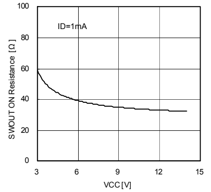
Fig.14. SWOUT ON resistance power supply property
