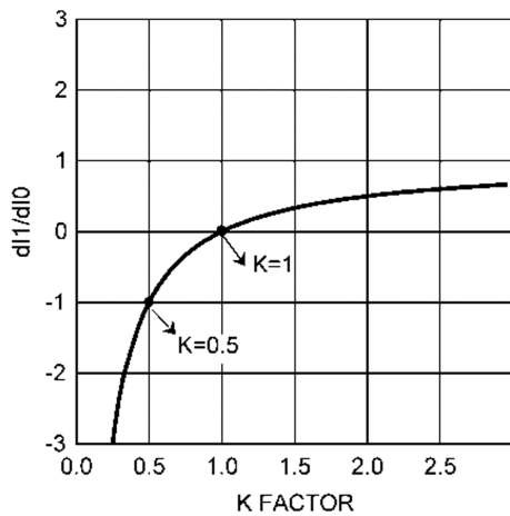
FIGURE 17. dl_1/dl_0 vs K Factor
