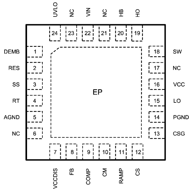
Top View LLP-24 (4mmx4mm)
