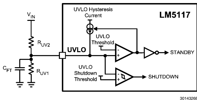
FIGURE 6. UVLO Configuration
