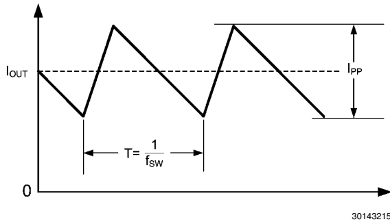
FIGURE 10. Inductor Current
