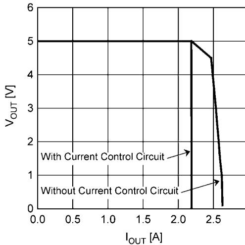
FIGURE 22. Current Limit Comparison
