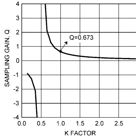
FIGURE 18. Sampling gain Q vs K Factor
