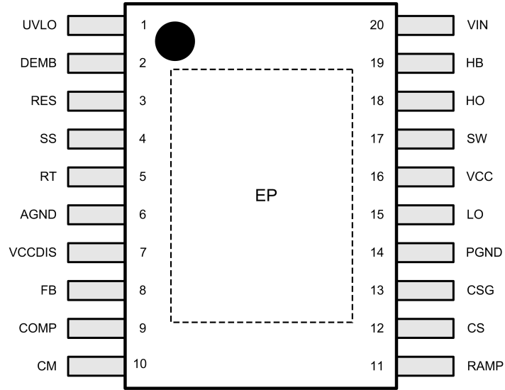
Top View 20-Lead TSSOP EP
