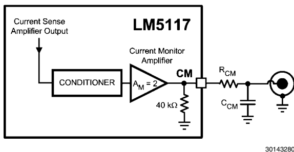
FIGURE 14. Current Monitor
