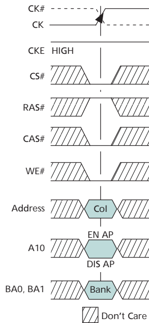
Figure 19: WRITE Command
