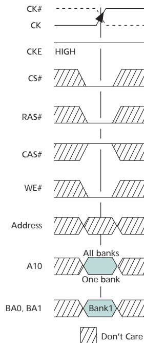
Figure 20: PRECHARGE Command
