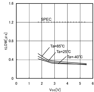
Fig. 15 Data clock "L" time tLOW
