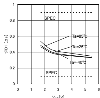
Fig. 21 Output data delay time tPD1
