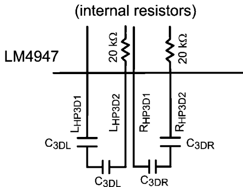
FIGURE 5. External 3D Effect Capacitors
