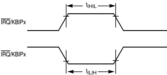
Figure 18. \overline{\text{IRQ}}/\text{KBIPx} Timing
