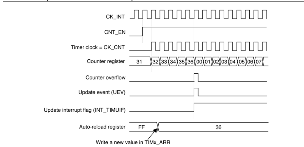
Figure 17. Counter timing diagram, update event when TIM_ARBE = 0 (TIMx_ARR not buffered)
