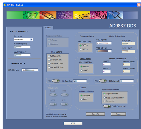
Figure 29. AD9837 Evaluation Software Interface
