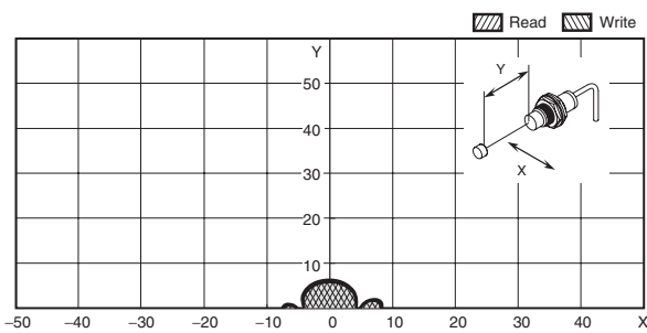
V680-HS51 (embedded in metallic material) & V680-D1KP52MT (embedded in metallic surface: steel)
