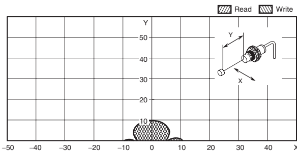
V680-HS51 (embedded in metallic material) & V680-D2KF52M (embedded in non-metallic material)
