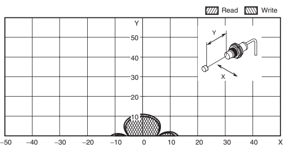
V680-HS51 (embedded in metallic material) & V680-D1KP52MT (embedded in non-metallic material)
