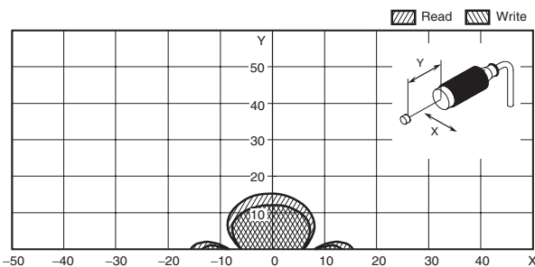
V680-HS51 (embedded in metallic material) & V680-D1KP52MT (embedded in non-metallic material)
