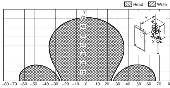
V680-HS63 (mounted on metallic material) & V680-D8KF68/-D32KF68 Mounted on metallic surface: steel (Vertical-facing ID Tag) When the V680-A81 ID Tag Attachment is mounted.
