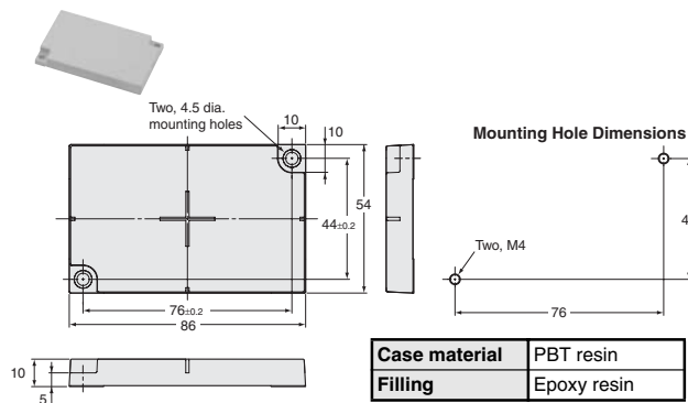
V680-D8KF68/-D32KF68
