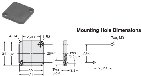
V680-D1KP66T/-D1KP66MT
