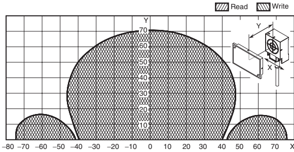
V680-HS63 (mounted on metallic material) & V680-D8KF68/-D32KF68 Mounted on metallic surface: steel (Horizontal-facing ID Tag) When the V680-A81 ID Tag Attachment is mounted.
