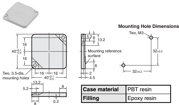
V680-D8KF68/-D32KF68
