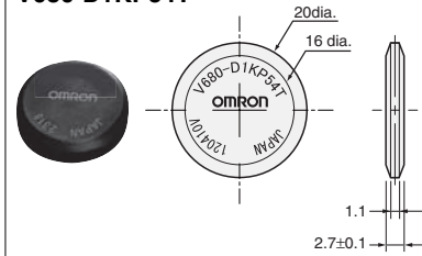
V680-D1KP54T
