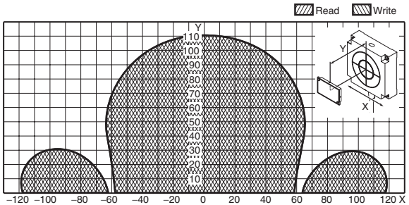
V680-HS65 (mounted on metallic material) & V680-D8KF68/-D32KF68 Flush-mounted on metallic surface: steel (Horizontal-facing ID Tag) When the V680-A81 ID Tag Attachment is mounted.
